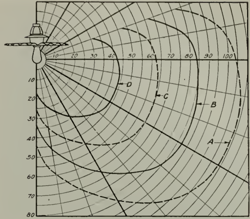
Fig. 3-b. Initial Distribution of Candle-power in a Vertical Plane of the Unit shown in Fig. 3-a
