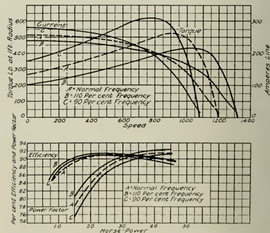
Fig. 3. Characteristic Curves at 10 per cent above and below normal frequency for the motor named in Fig. 1
