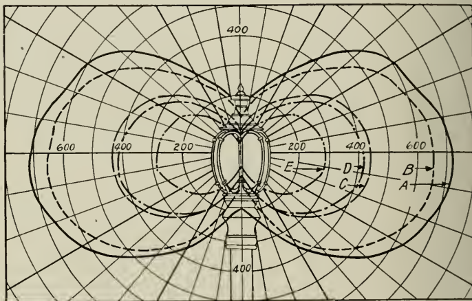
Fig. 14-b. Initial Distribution of Candle-power in a Vertical Plane of the Unit shown in Fig. 13-a
