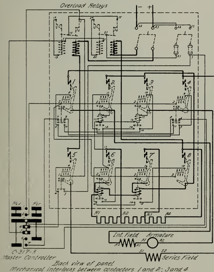
Fig. 14. Connection Diagram of a Starting Panel for Direct-current Motors Using Current-limit Interlocks
