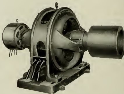
Fig. 2. Form PB Alternator with Direct-connected Exciter
