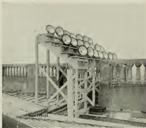
Fig. 2. One of Four Banks of Flood Lighting Projectors for Illuminating Dome
