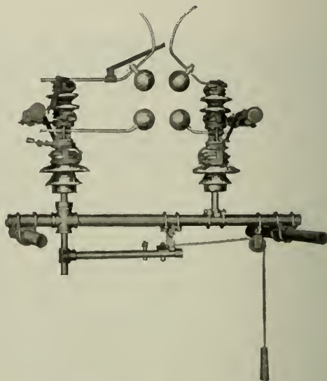
Fig. 7. Sphere-horn Gap for use with 20,000 Volt Aluminum Arrester
