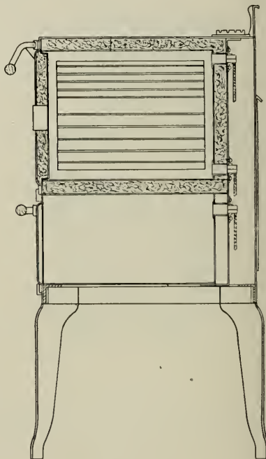
Fig. 4. Cross Section of an Electric Range
