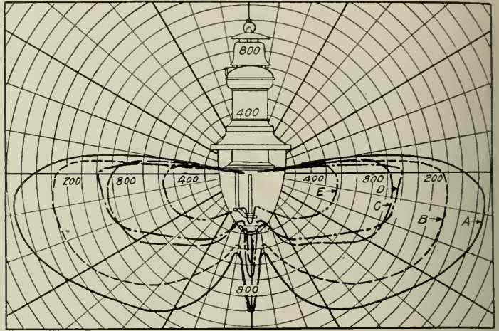
Fig. 9-b. Initial Distribution of Candle-power in a Vertical Plane of the Unit shown in Fig. 9-a
