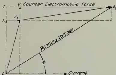
Fig. 17. Voltage Diagram of the Plain Series Motors
