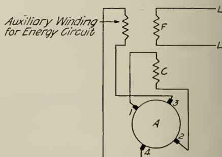
Fig. 62. Adjustable Speed Repulsion Induction Motor with Energy Secondary
