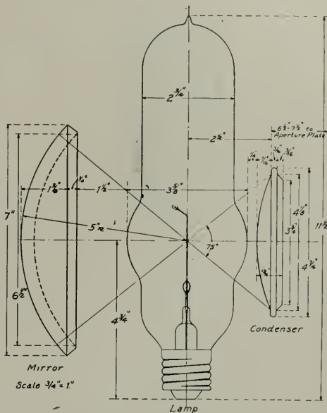
Fig. 6. 30-Ampere Motion-Picture Lamp, Corrugated Condenser, and Spherical Mirror in Correct Operating Positions
