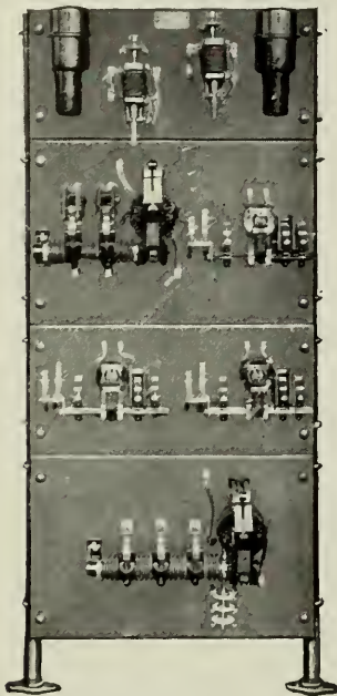
Fig. 5. Current-limit Starting Panel for an Induction Motor with Form-wound Rotor
