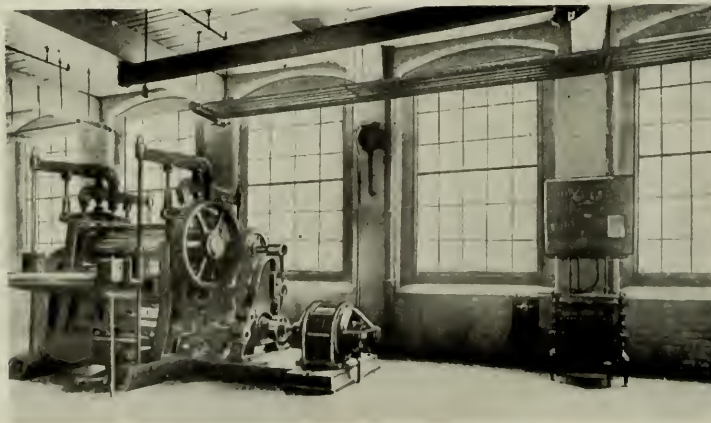
Fig. 28. 15-h.p., 600-r.p.m., 550-volt Slip Ring Induction Motor and Panel for Plater
