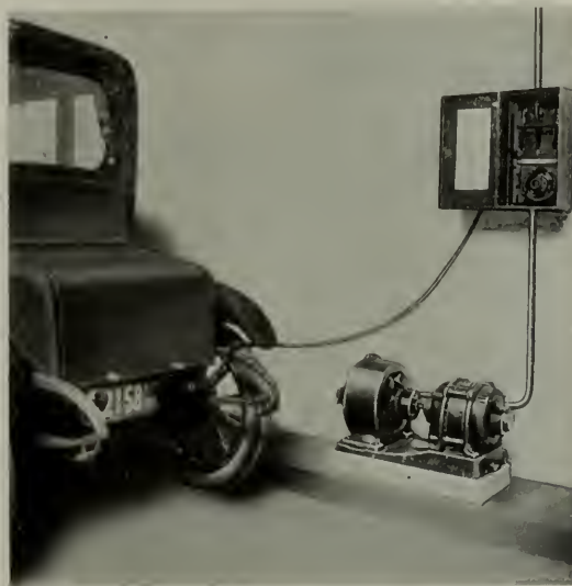
Fig. 13. Standard Taper Individual Vehicle Charging Equipment
