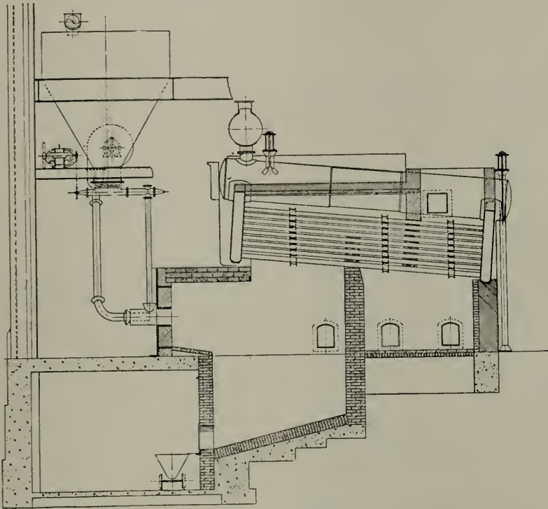
Fig. 9. Boiler in the Shops of the Missouri, Kansas & Texas Railroad Company, Parsons, Kansas. Converted from oil firing to low-grade pulverized coal firing
