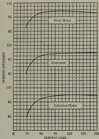
Fig. 3. Efficiency Curves
