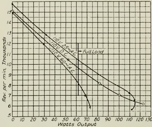
Fig. 18. Output Curves of \frac{1}{2} h.p., 8000 r.p.m., 110-volt Universal Motor
