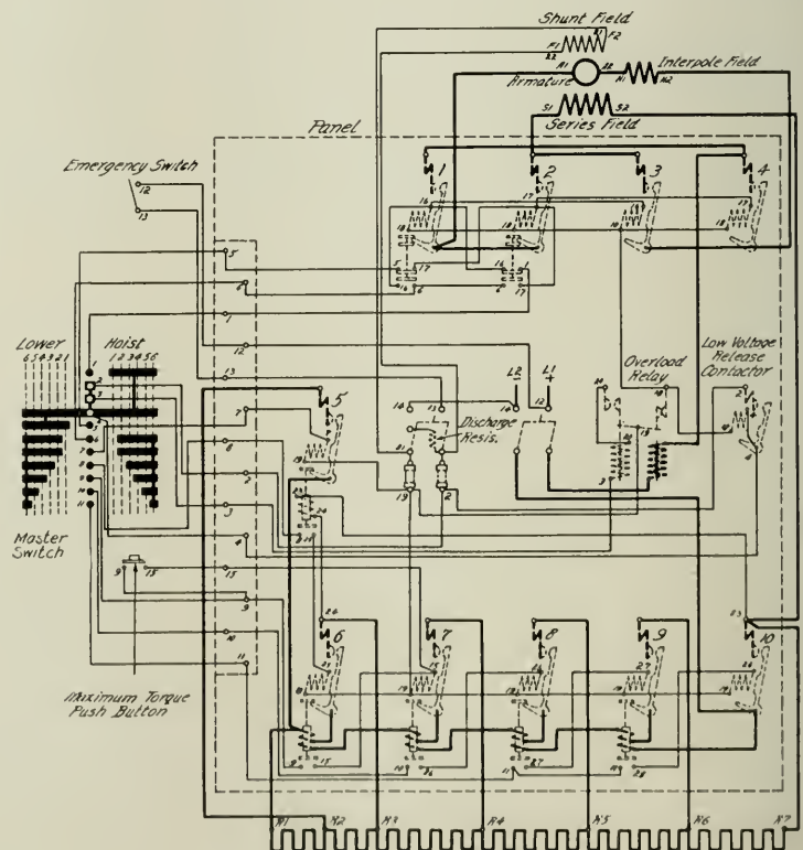
Back view of panel Mechanical interlocks between contactors 1 and 2; 3 and 4
