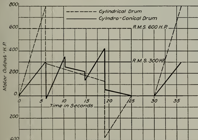
Fig. 2. Comparison of Load Diagram with Cylindrical Drum and CyIndro-conical Drum
