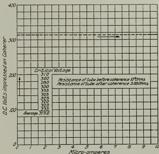
Fig. 8. Volt-Ampere Characteristic Curve of G-E Coherer No. 1065
