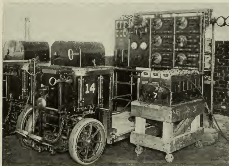
Fig. 2. Switchboard Serving Industrial Trucks in a Factory
