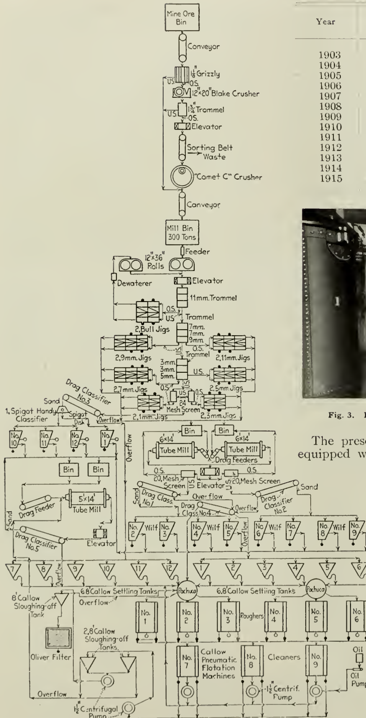
Fig. 2. Flow Sheet of Mill at Gold Hunter Mine. This Method of Handling Ore Represents Practically Standard Practice
