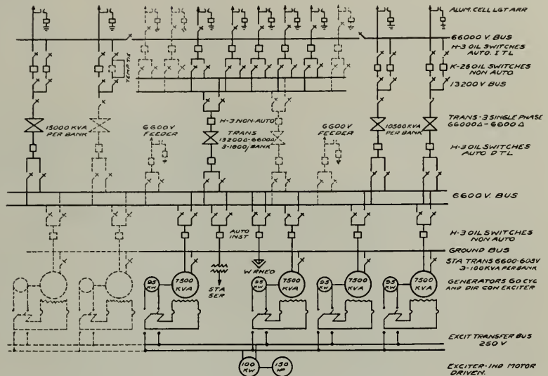
Fig. 12. Diagram of Station Connections
