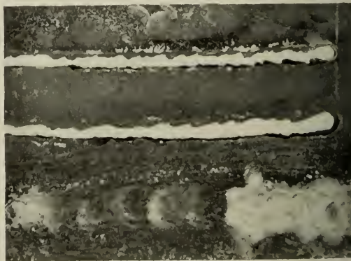
Fig. 3. Two Pieces of Steel Plate Joined by Electric Arc Welding. Carbon Electrode Used. Also Appearance of Cuts Made by Carbon Electrode
