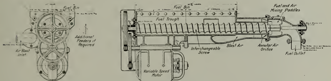
Fig. 6. Pulverized fuel feeder
