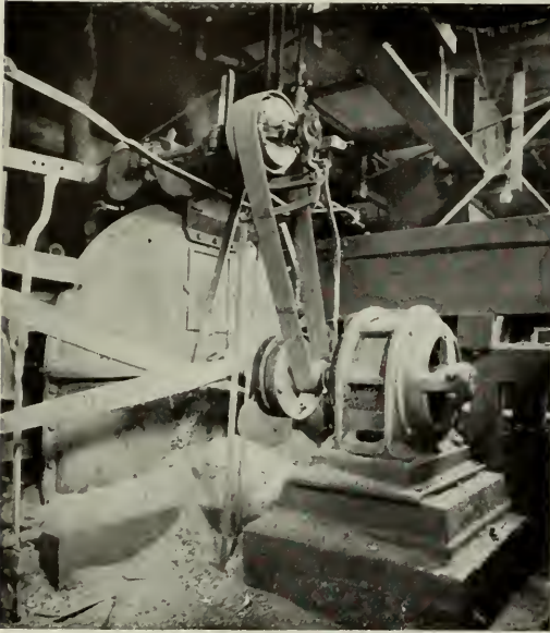
Fig. 5. 15-h.p., 750-r.p.m., 440-volt Form K Induction Motor driving 5-ft. barker. Kimberly-Clark Company, Kimberly, Wis.
