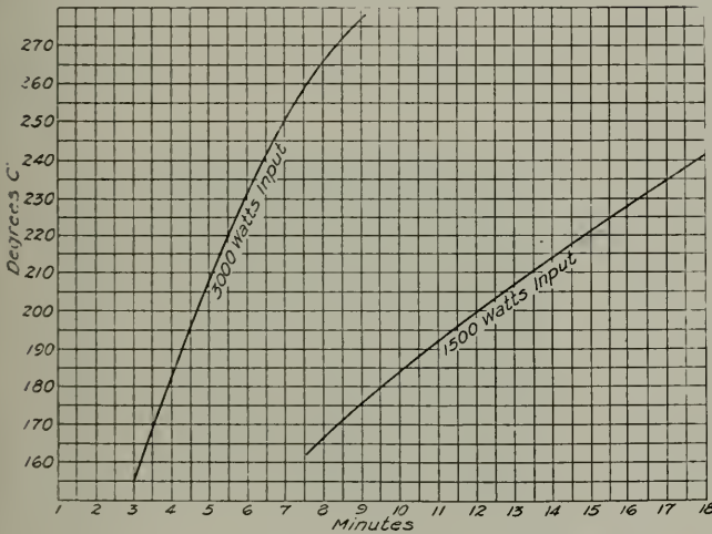
Fig. 12. Time to Preheat a Standard Oven 18 Inches by 28 Inches by 14 Inches
