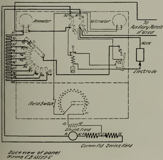
Fig. 5. Connections of Arc Welding Control Panel for Controlling Generator and One Welding Circuit
