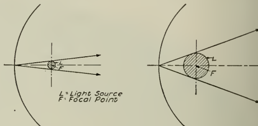
Fig. 3. Illustrating Influence of Size of Light Source on Spread of Beam
