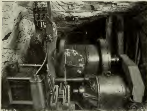
Fig. 9. Hoist, made by Connellsville Mfg. & Mine Supply Company, has 36-in. drum, double gear reduction, one reduction being obtained by back geared motor rated at 30 h.p. intermittent service, fully enclosed
