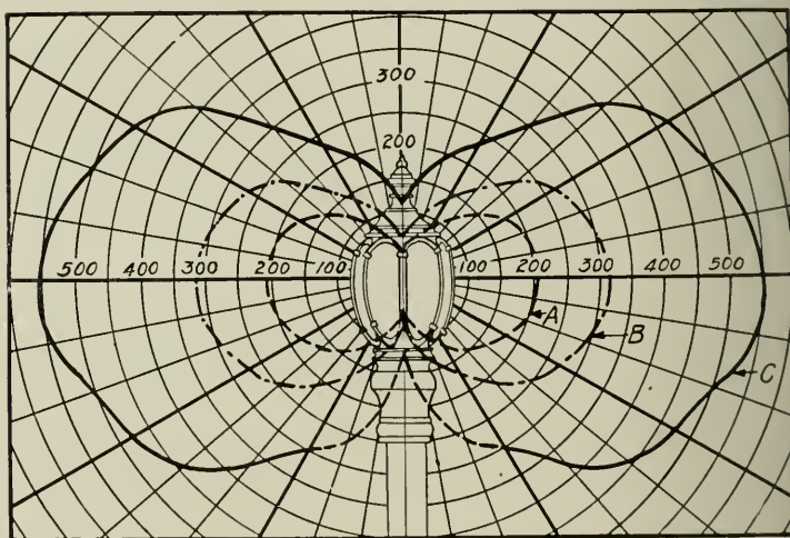
Fig. 8-b. Initial Distribution of Candle-power in a Vertical Plane of the Unit shown in Fig. 8-a
