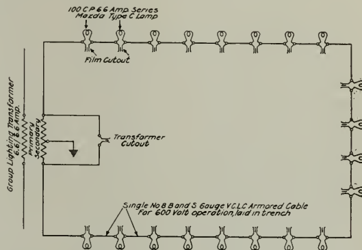
Fig. 2. Secondary Lamp Circuit
