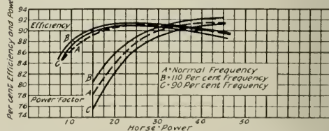
Fig. 3. Characteristic Curves at 10 per cent above and below normal frequency for the motor named in Fig. 1
