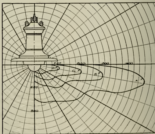
Fig. 6-d. Initial Distribution of Candle-power in a Vertical Plane of the Unit shown in Fig. 6-c Curves A, B, C and D correspond to the lamps named in Fig. 6-c
