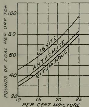
Fig. 4. Fuel required for drying
