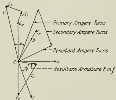
Fig. 20. Vector Diagram of Repulsion Motors
