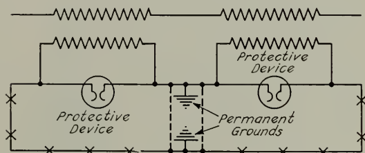
Fig. 3. Diagram of Series Circuit Employing Two Similar Series Transformers with Intermediate Point Between Secondaries and Middle Points of Lamp Circuit Grounded and with Two Protective Devices in Circuit
