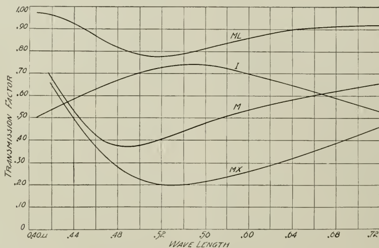
Fig. 1. Spectral Transmission of Different Kinds of Glasses
