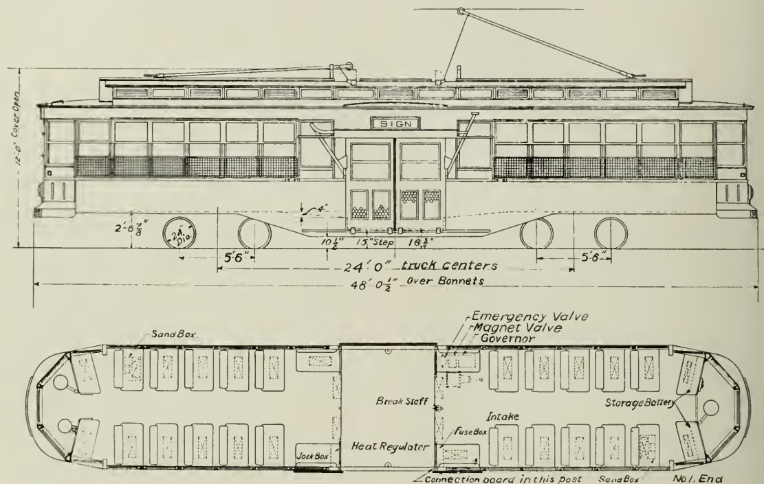
Fig. 1. Elevation and Plan of New Cars
