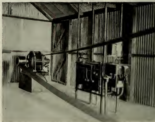
Fig. 4. A California installation of an oil well motor of the Y-delta type
