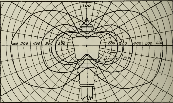
Fig. 7-b. Initial Distribution of Candle-power in a Vertical Plane of the Unit shown in Fig. 7-a Curves A, B, C and D correspond to the lamps named in Figs. 7-c and 7-d.
