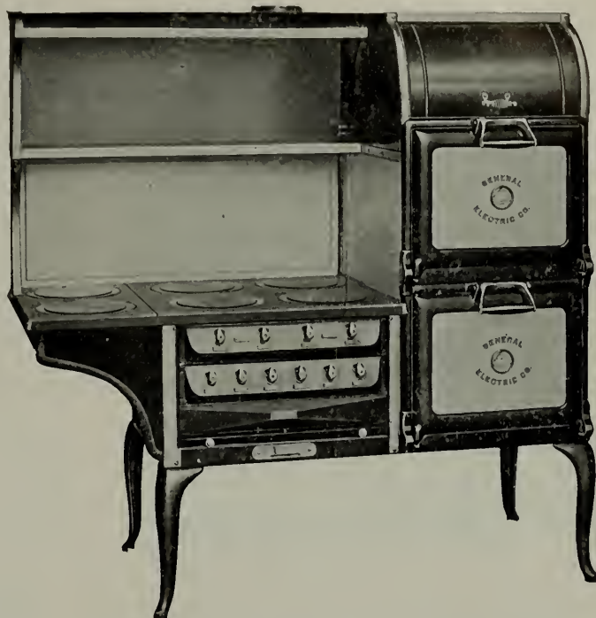
Fig. 5. Electric Range with Four Eight-inch and Two Six-inch Hot Plates, Two Ovens with Two Units Each, and a Warming Closet. All units are of the three-heat type
