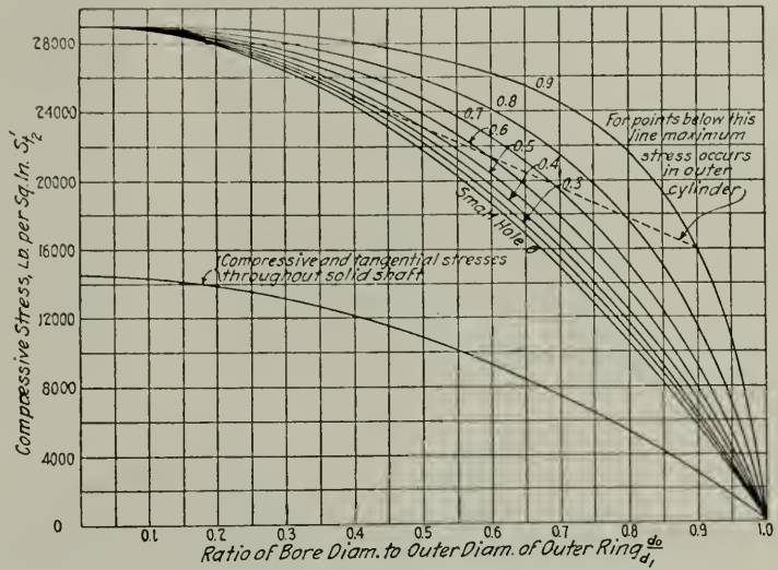
Fig. 3. Compressive Tangential Stress S'_{t2} at Inner Diameter of Inner Ring. Force Fit of 0.001 In. Per In. of Bore. Both Parts Steel
