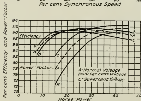
Fig. 2. Characteristic Curves at 10 per cent above and below normal voltage for the motor named in Fig. 1
