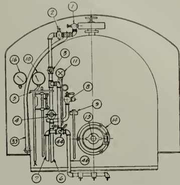
VIEW SHOWING RIGHT OF CAB EQUIPMENT
