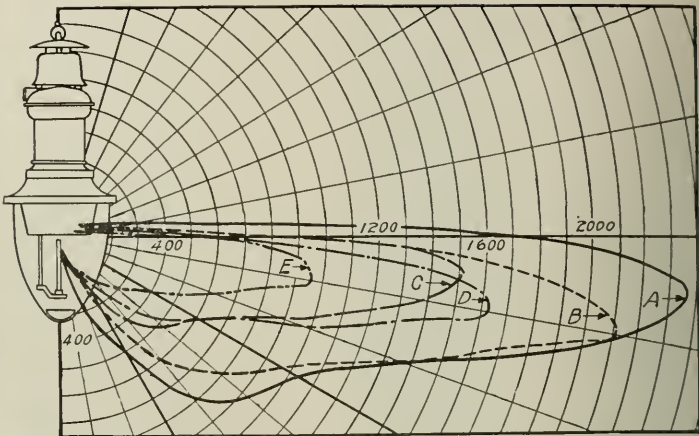
Fig. 11-b. Initial Distribution of Candle-power in a Vertical Plane of the Unit shown in Fig. 11-a Curves A, B, C, D and E correspond to the currents and electrodes named in Fig. 11-c.
