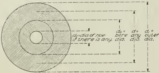
Fig. 5. Diagram of a Force Fit of a Hub or Ring over a Solid or Hollow Shaft
