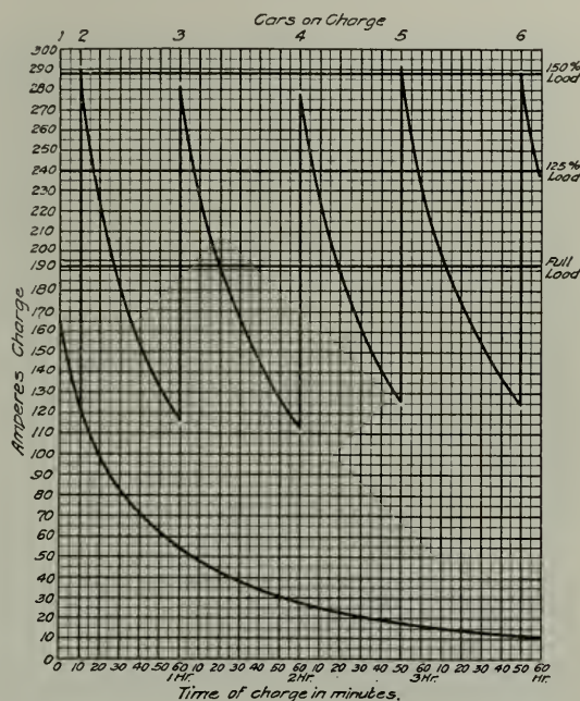
Fig. 3. Theoretical Curves showing Constant-potential Characteristics of a 13-plate "Hycap Exide" cell and the result of loading a generator with six such batteries at stated intervals
