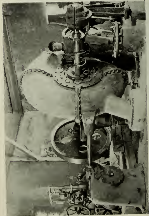
Fig. 9. Hydraulic Turbine
