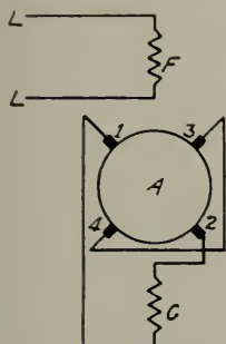
Fig. 37. Compensated Repulsion Induction Motors, Type RI
