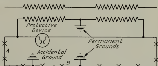
Fig. 2. Diagram of Series Lighting Circuit Employing Two Similar Series Transformers with Intermediate Point Between Secondaries and Middle Point of Lamp System Grounded
