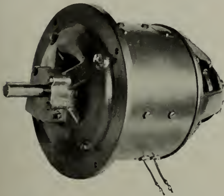
Fig. 14. Motor Suitable for Band Saw Drive, Mounring Lower Wheel Directly on the Shaft
