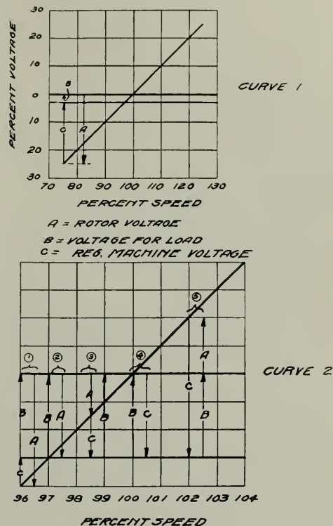
Fig. 5. Curves of Speed vs. Secondary Voltage Through Synchronism Resolved into Their Component Voltages
