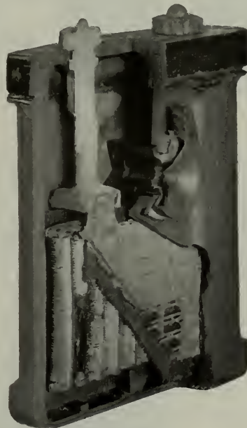
Fig. 7. The Ironclad Exide Battery
