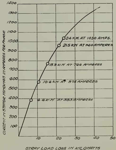
Fig. 7. Stray Load Loss of Generator
