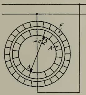
Fig. 38. Bipolar Repulsion Motors
