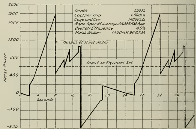
Fig. 16. Duty Cycle of 1400-h.p. 90-r.p.m. Motor Operating on Ilgner Ward Leonard System with Motor-generator Set Consisting of 1000-kw. Generator and 600-h.p. Induction Motor Coupled to 30,000-lb. Flywheel
