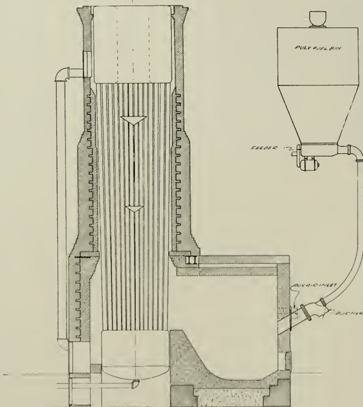
Fig. 2. Application of pulverized fuel Cahall boiler
