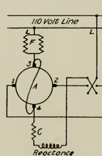
Fig. 55. Connections for Reversing Standard Type R1, 110-volt Motors
