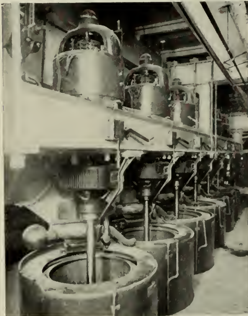
Fig. 10. Motor Built-in Sugar Centrifugals. Individual Drive for sugar centrifugals is usually accomplished by horizontal motor and quarter-turn belt for each centrifugal
