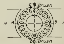
Fig. 15. Distribution of Electromotive Forces in Armature
