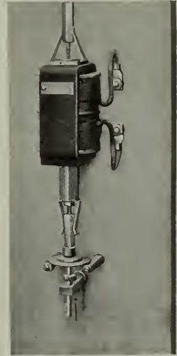
Fig. 12. Alternating-current Step-back Relay
