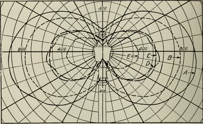
Fig. 13-b. Initial Distribution of Candle-power in a Vertical Plane of the Unit shown in Fig. 13-a Curves A, B, C, D and E correspond to the currents and electrodes named in Figs. 13-c and 13-d.
