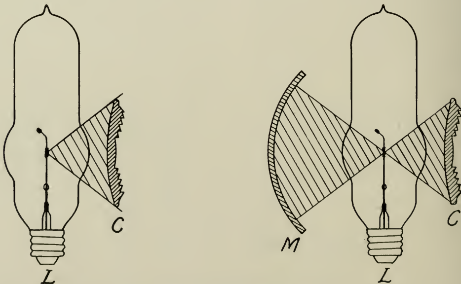
Fig. 4. Arrangement of Lamp, Mirror, and Condenser
