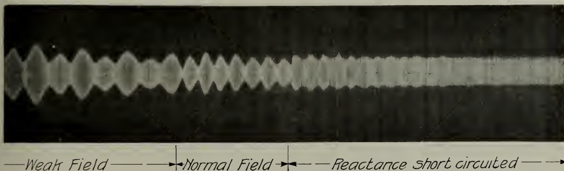
Fig. 10 (Cont'd) The length of the Oscillogram is equivalent to about 15 seconds and extends from the time the generator was first connected to the line to the time the machine is satisfactorily carrying its share of the load
