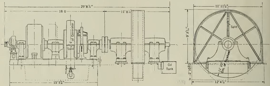
Fig. 5. Outline of Motor-Generator Set
