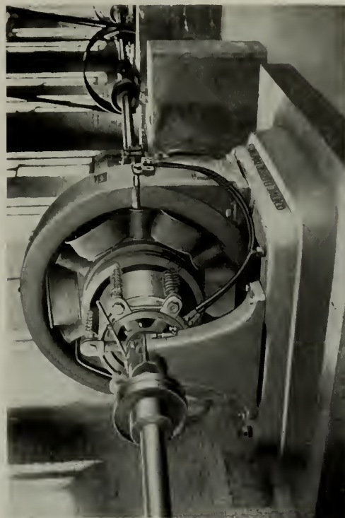
Fig. 21. One 100/225-h.p., 275/500-r.p.m., 220-volt Variable Speed Direct Current Motor direct-connected at both ends to line shafting driving variable speed end of paper machine. Consolidated Water Power and Paper Company, Grand Rapids, Wis.
