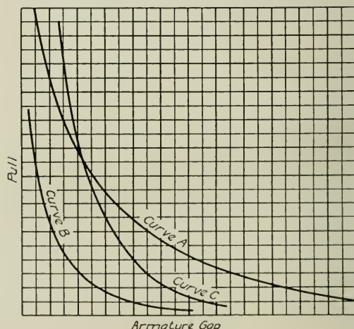
Fig. 1. Curve showing Variation of Pull on Armature of Solenoid at Different Air Gaps, for Alternating Current and Direct Current
