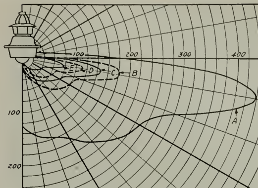
Fig. 5-b. Initial Distribution of Candle-power in a Vertical Plane of the Unit shown in Fig. 5-a
