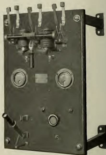
Fig. 15. Individual Vehicle Charging Panel with Automatic Protection for use when ampere-hour meter is installed on the vehicle
