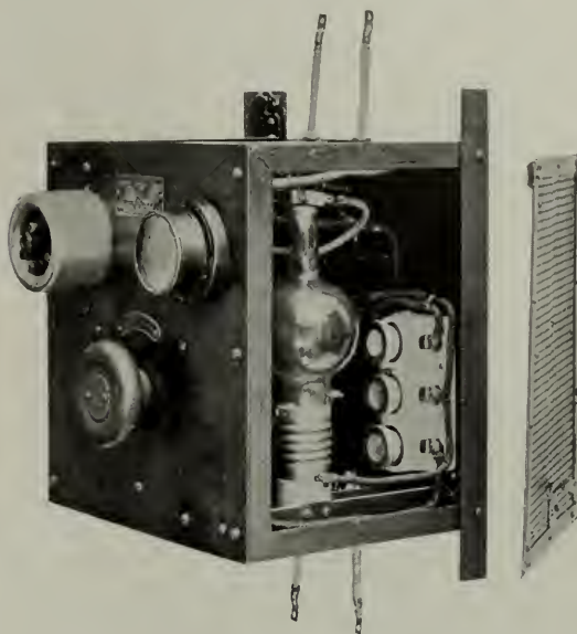
Fig. 9. Six-ampere, 75-volt Rectifier with side grating removed, showing Tungar Bulb and Fuse Block
