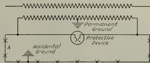
Fig. 1. Diagram of Series Lighting Circuit Employing Single Series Transformer with Middle Point of Secondary Grounded
