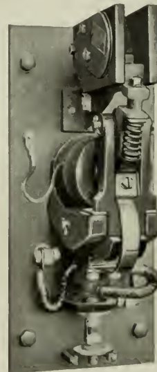
Fig. 2. 600-Volt, 339-Amp. Direct-current Contactor with Series Current Limit Interlock
