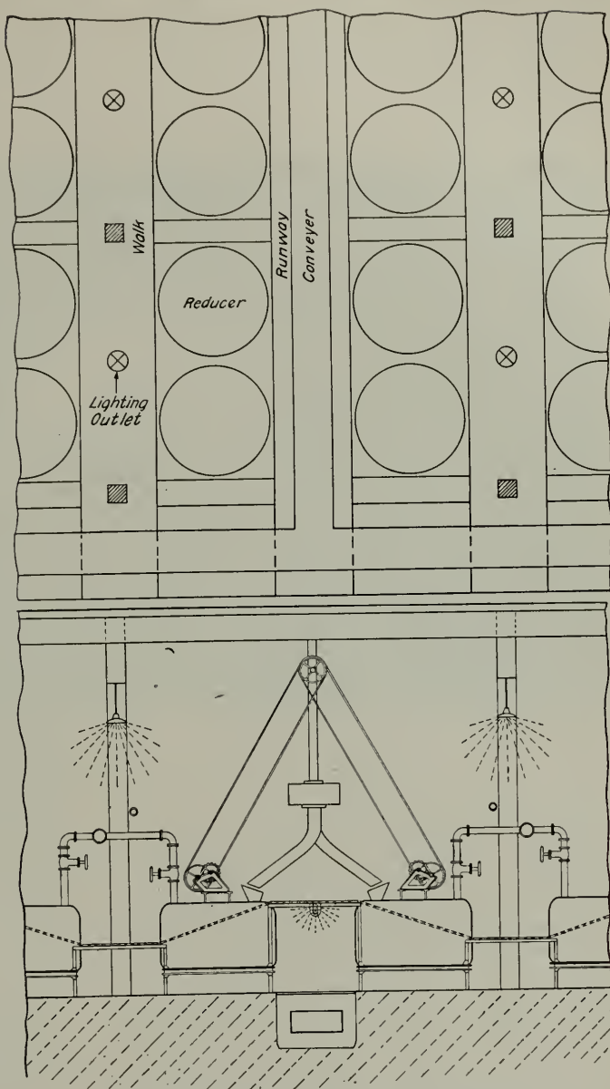
Fig. 1. Plan and Elevation of Portion of Reducer Plant Showing Arrangement of Reducers and Lighting Units
