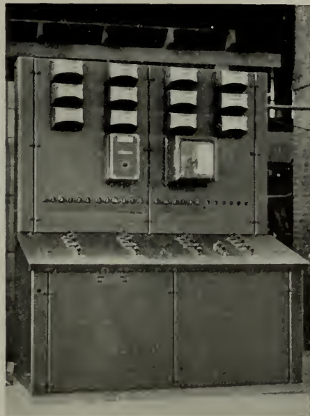
Fig. 9. Benchboard on which are Mounted all the Indicating and Totalizing Meters and supplementary Remote Control Equipment of the Hydro-electric Station. This Benchboard is located in the Main Generating (steam) Station
