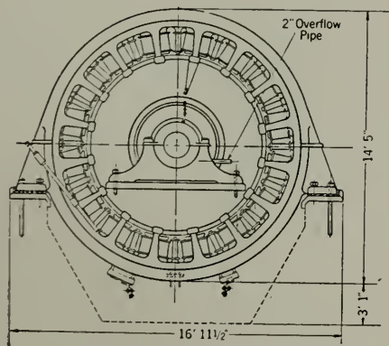
Fig. 4. Outline of Hoist Motor
