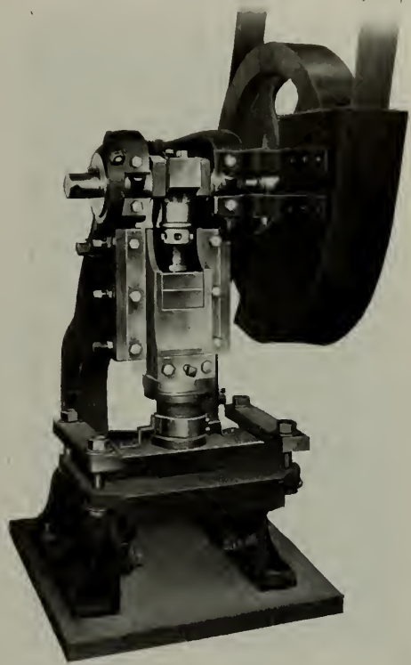
Guard on press for punching mica washers. Front of guard is covered with transparent mica which permits the operator to see the work but prevents the fingers being put under die
