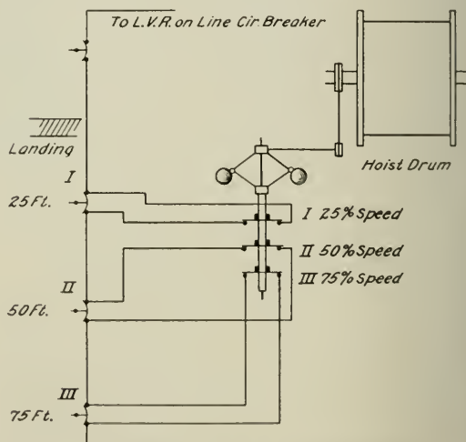
Fig. 7. Diagram of Apparatus for Protection against Overwinding
