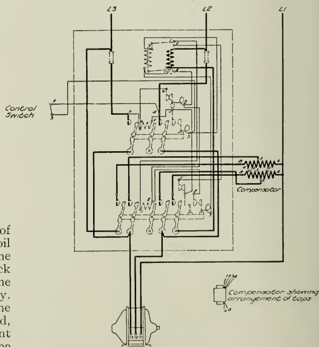
Fig. 2. Connection Diagram of the Automatic Compensator Panel shown in Fig. 1
