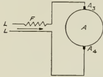
Fig. 13. Circuit of Plain Series Motors
