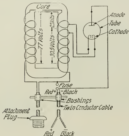
Fig. 6. Complete Connection of Two-ampere Rectifier
