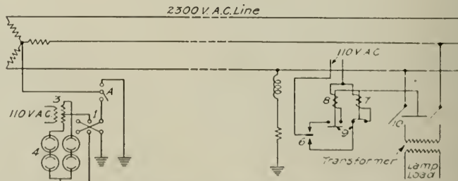
Fig. 2. Connection Diagram of Phantom Circuit Remote Control System, as applied to a Grounded Neutral Line
