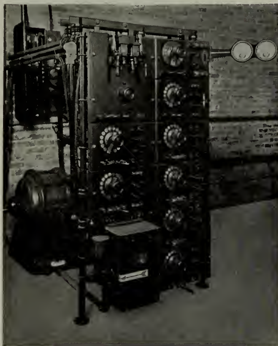
Fig. 9. Charging Equipment in a Public Garage
