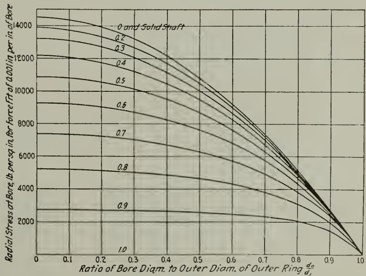
Fig. 4. Radial Stress at Bore S_r . Force Fit of 0.001 In. Per In. of Bore. Both Parts Steel
