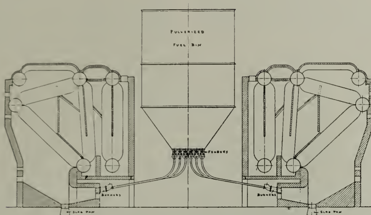
Fig. 3. Application of pulverized fuel Badenhausen boiler
