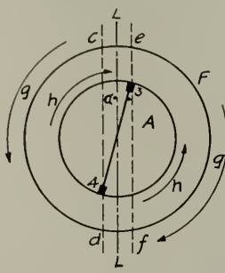
Fig. 39. Working Diagrams of Bipolar Repulsion Motors
