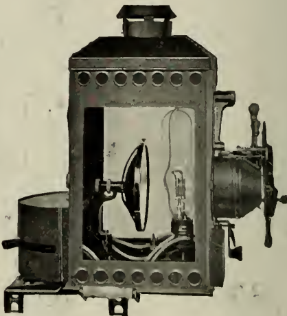
Fig. 8. Lamp Housing, showing Arrangement of Mirror, Lamp, and Condenser
