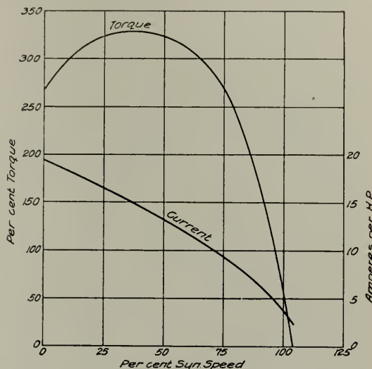
Fig. 45. Speed-torque and Speed-current Curves of a Typical Type RI, Single-phase Constant-speed Motor
