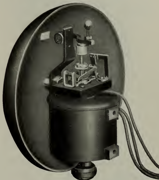
Fig. 2. Counter-Gong Relay for Coherer Discharge Alarm
