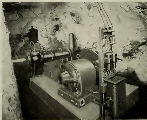
Fig. 5. Typical Bottom Pump Installation showing 5 by 7 Aldrich Triplex Pump Driven by Fully Enclosed 15-h.p. Squirrel-cage Induction Motor through Flexible Coupling
