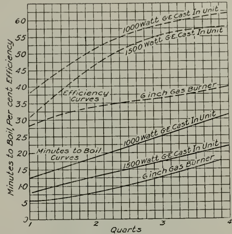
Fig. 13. Minutes to Boil and Efficiencies on Different Hot Plates and a Gas Burners Using a Four-quart Cast Aluminum Kettle
