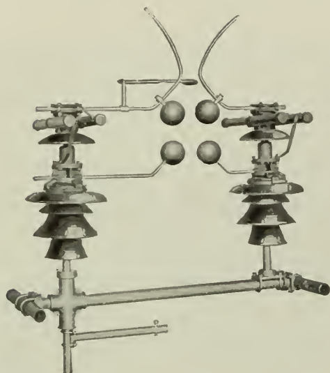
Fig. 5. Sphere-horn Gap for use with 70,000 Volt Aluminum Arrester
