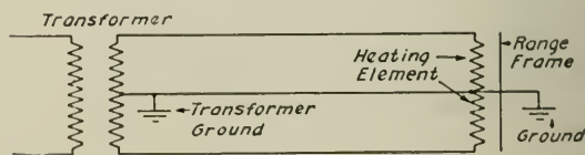
Fig. 11 Diagram showing the Grounding of the Neutral and the Range Frame
