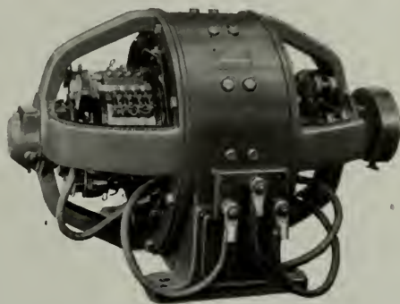
Fig. 26. 100-kw. 1200-r.p.m. 250-volt Three-wire Synchronous Converter
