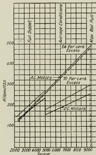
Fig. 5. Kw. Input Curves of Direct-current and Alternating-current Motors Operating under Conditions similar to those in Fig. 4
