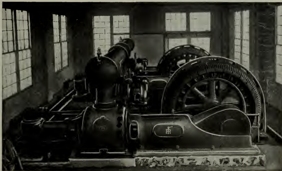
Fig. 1. Motor Built-in Applied to Air Compressor
