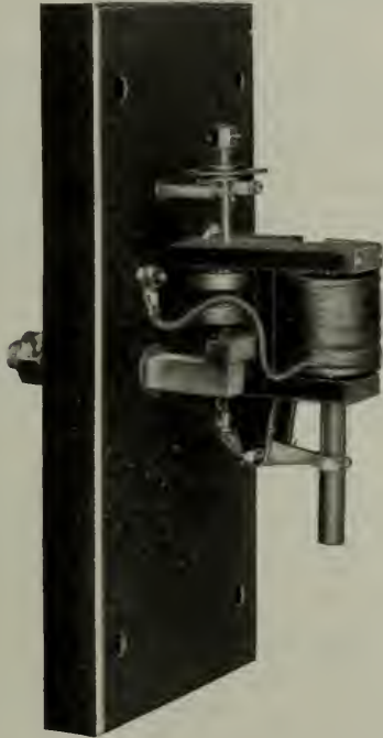
Fig. 10. Current Limit Alternating-current Relay
