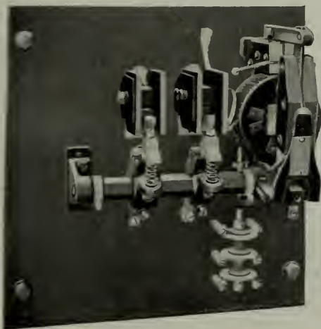
Fig. 3. 600-Volt, 150-Amp., D. P. Alternating-current Contactor
