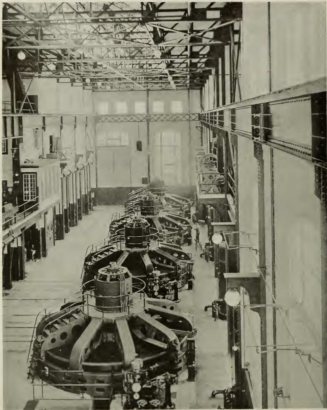
Fig. 6 Interior of Power House showing the 7500-Kv-a. Generators
