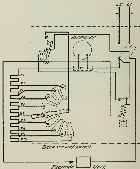
Fig. 23. Connection Diagram of the Auxiliary Arc Welding Panel shown in Fig. 22
