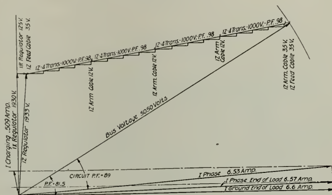
Fig. 5. Vector Diagram of Currents in Group Street Lighting Circuit
