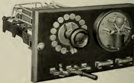
Fig. 11. Series-rheostat Section with Automatic Protection Device
