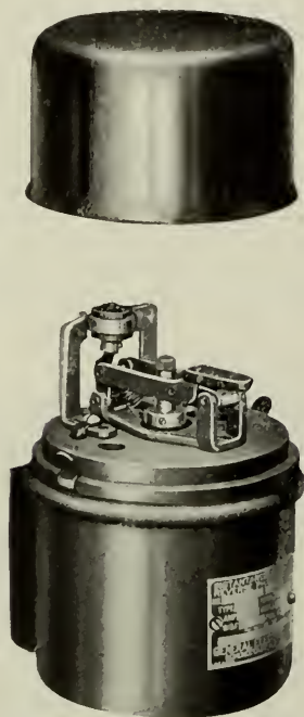
Fig. 3. Reverse Phase Relay
