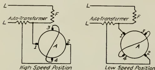
Fig. 29. Varying Speed Brush-shifting Motors, Type BSS
