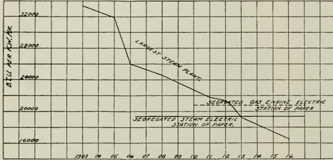
Fig. 14. Heat Consumption, in B.t.u. per Kw.-hr., for Complete Electric Stations on Steady Load. The figures in all cases include all power-plant apparatus, including auxiliaries and emergency reserves
