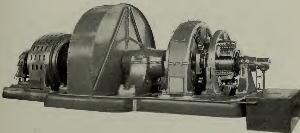
Fig. 14. Motor-generator Set of Ilgner Ward Leonard System
