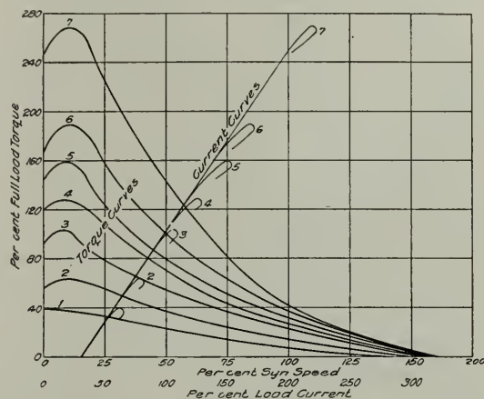
Fig. 21. Torque-speed and Torque-current Curves for Different Values of Resistance in Series with a 7\frac{1}{2} h.p., 1200 r.p.m., 220-volt, Crane and Hoist Motor
