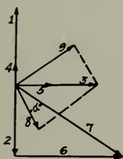
Fig. 44. Vector Diagram of Compensated Repulsion Induction Motor
