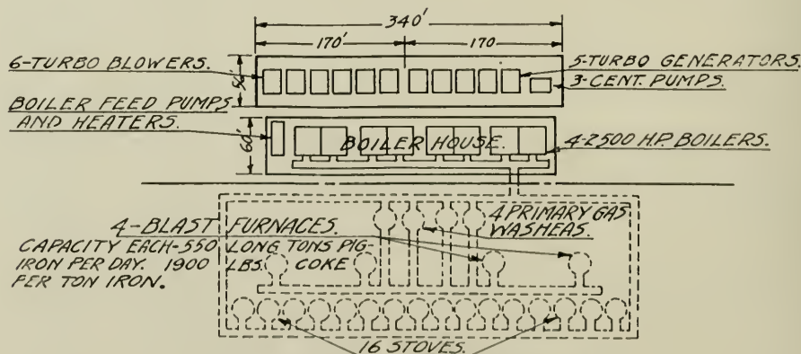
Fig. 17. Layout of Four-furnace Steam-turbine Plant
