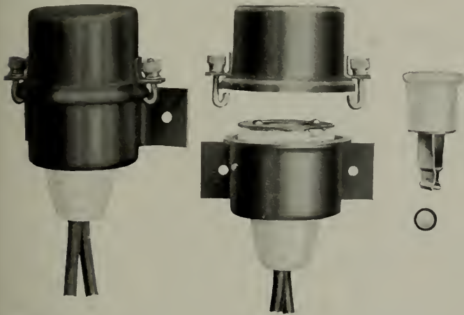
Figs. 6 and 7. Views of Protective Device, Assembled and Disassembled
