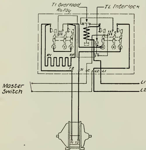
Fig. 10. Connection Diagram of the Time-limit Starter shown in Fig. 9
