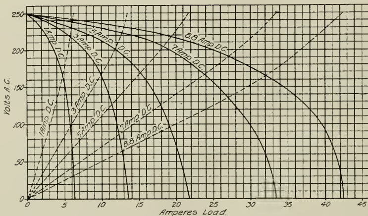
Fig. 2. Test curves made with the set-up in Fig. 1 to show the relation between the voltage across a varying load and the load (full curves), also between the voltage across the reactance and a varying load (dotted curves). Alternator supply held at 250 volts and 125 cycles. Direct-current excitation held constant for each curve
