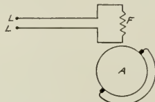
Fig. 4. Circuit of Plain Repulsion Motor (Thomson Repulsion Motor)
