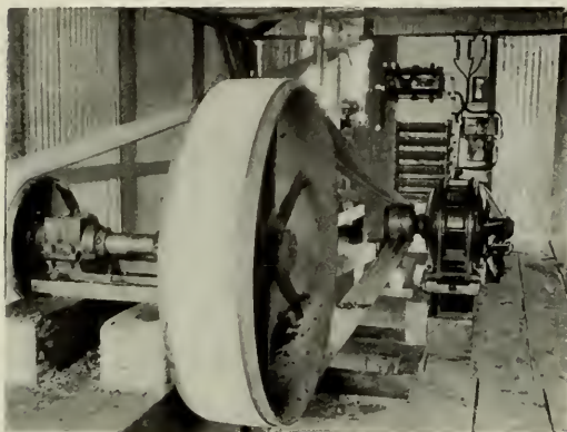
Fig. 3. Two-speed variable-speed 25 \frac{8}{8} h.p. oil well motor installation for pumping, pulling and cleaning work in the Midway field in California
