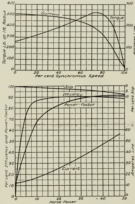
Fig. 1. Characteristic Curves of a 30-h.p., 3-phase, 60-cycle, 440-volt, 1200-r.p.m. Motor
