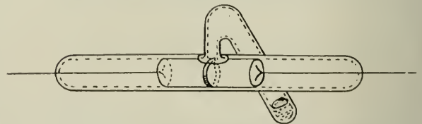
Fig. 6. Blondel Side-Pocket Metallic Filings Coherer
