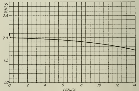
Fig. 4. Voltage Characteristic Curve of Ironclad Exide Battery
