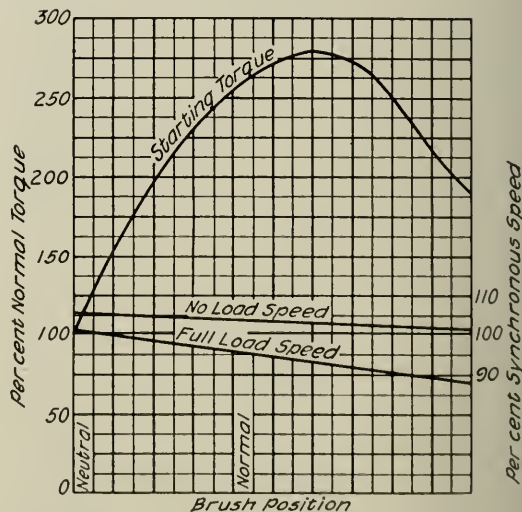
Fig. 49. Effect of Shifting Brushes on Constant Speed, Type RI Motors
