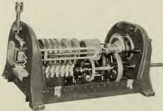
Fig. 12. Controller Used with the Ilgner Ward Leonard System
