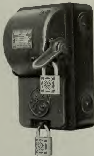
Fig. 32. Enclosed "Safety First" Lever Switch, 2-pole, 30-amp. 250-volt, Switch Locked Open, Fuse Compartment Locked Closed
