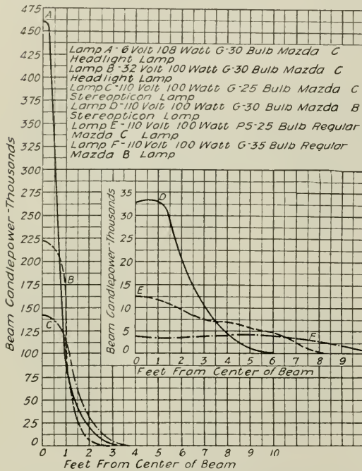
Fig. 7. Distribution Curves of Lamps Shown in Fig. 6.
