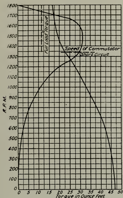
Fig. 35. Speed-torque Curves of \frac{1}{4} h.p., 1800-r.p.m., Single-phase, 60-cycle, 110/220-volt Repulsion Induction Motor, Type RSA
