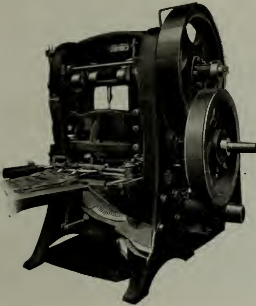
Automatic mechanical feed for punch press which makes it unnecessary for operator to put his hands anywhere near the die while machine is in motion
