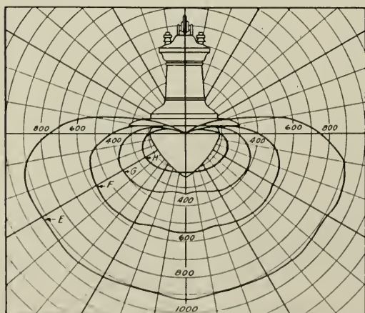
Fig. 6-b. Initial Distribution of Candle-power in a Vertical Plane of the Unit shown in Fig. 6-a Curves E, F, G and H correspond to the lamps named in Fig. 6-c.
