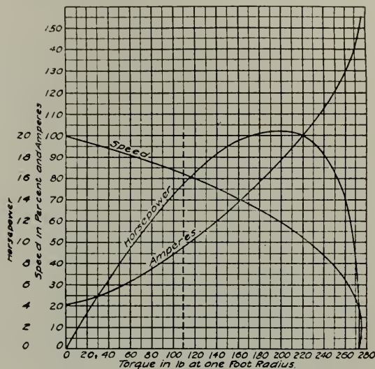
Fig. 58. Performance Curves of a Polyphase Reversible Motor
