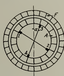
Fig. 40. The Commutator Induction Motor
