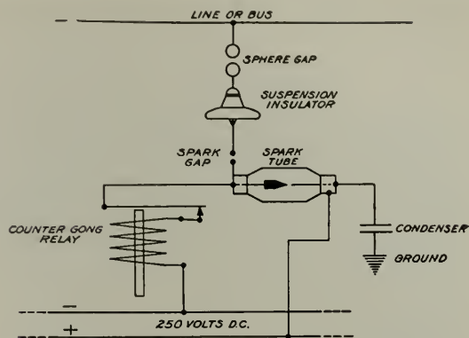
Fig. 12. Wiring Diagram for Spark-tube Surge Recorder
