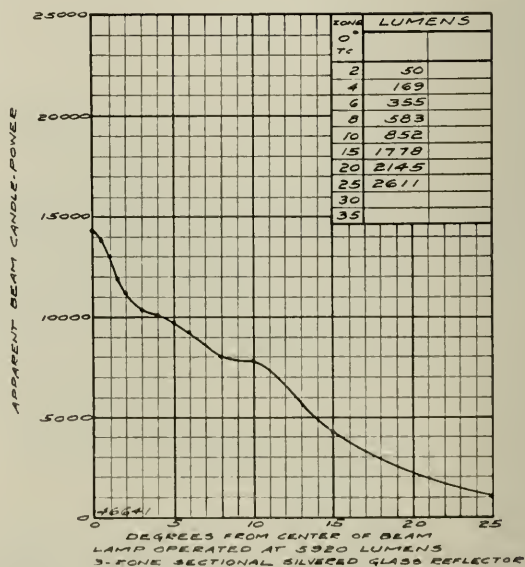
Fig. 6. Curve showing the initial distribution of candle-power in a horizontal plane from a Form L3 flood light projector with 400-watt Mazda C flood lighting lamps
