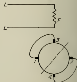
Fig. 23. Circuits of One Type of Déri Brush Shifting Motors
