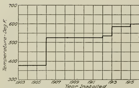
Fig. 6. Initial Temperatures Used in Large Steam Turbines
