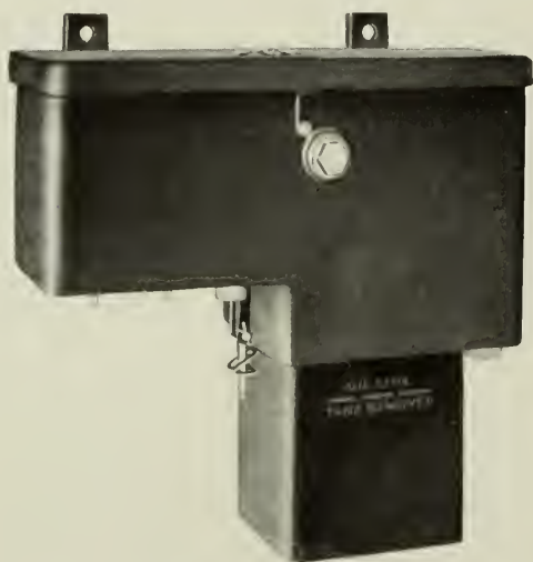
Fig. 1. Automatic Oil Switch for Connecting and Disconnecting Street Light Circuits to Feeders
