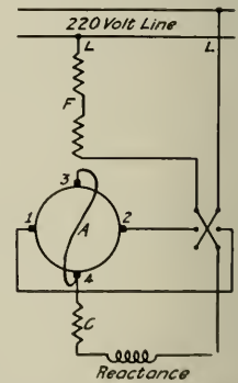
Fig. 56. Connections for Reversing Standard Type R1, 220-volt Motors
