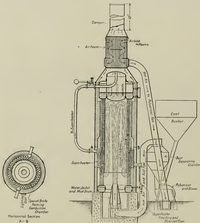
FIG. 8 BETTINGTON BOILER
