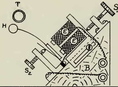
Fig. 5. Marconi's Electromagnetic Tapper for tapping his Sensitive Tube to a Receptive Condition. E, E, Electro-magnet; H, Hammer; T, Sensitive Tube shown in Cross Section; S 1 , S 2 , Adjusting Screws
