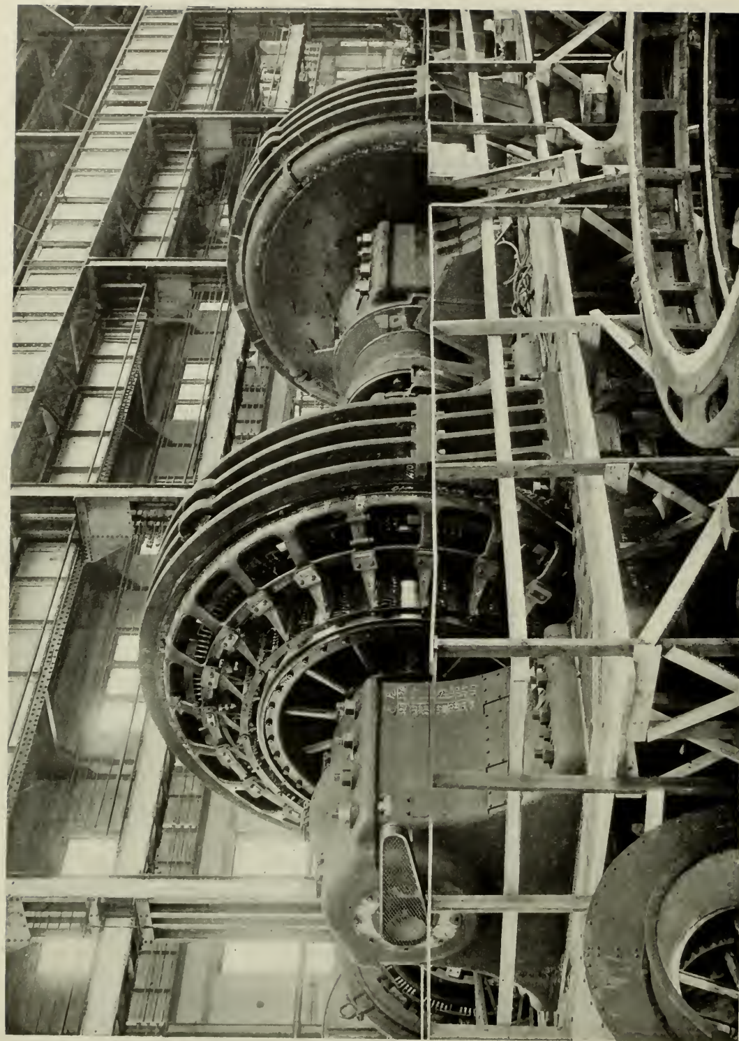
TWO REVERSING MOTORS FOR STEEL ROLLING MILL, COUPLED TOGETHER FOR LOCAL TEST
