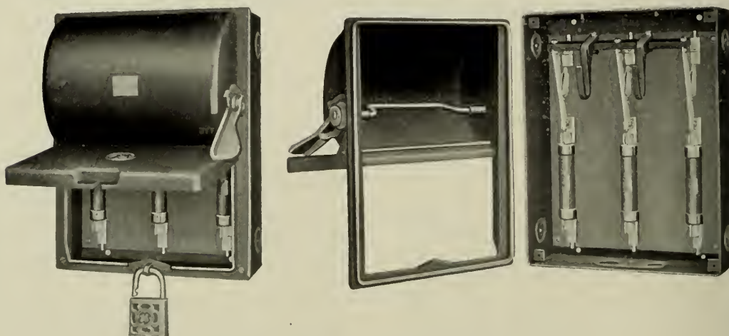
Fig. 4. Safety First Enclosed Lever Switch, showing Quick Break Parts
