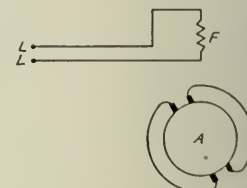
Fig. 8. Circuit of Déri Brush Shifting Motor
