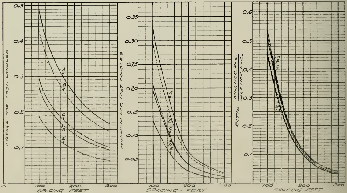
Fig. 9-c. Calculated Illumination Values on Street Surface along Center Line of Street
