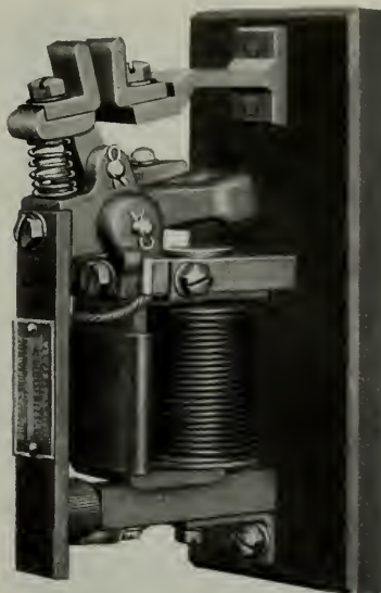
Fig. 4. 600-Volt, 75-Amp. Series Contactor
