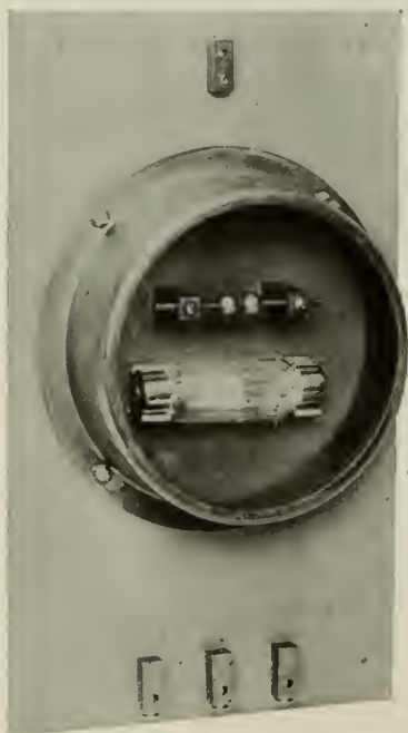
Fig. 9. Spark Tube Panel for Spark-tube Discharge Alarm
