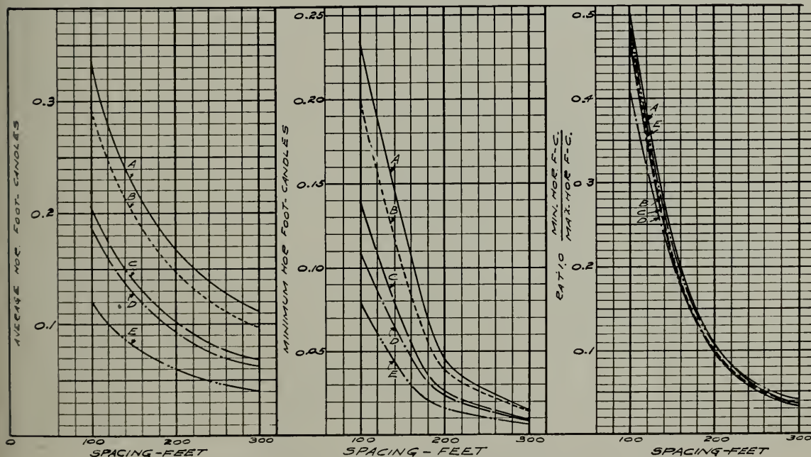
Fig. 10-c. Calculated Illumination Values on Street Surface along Center Line of Street
