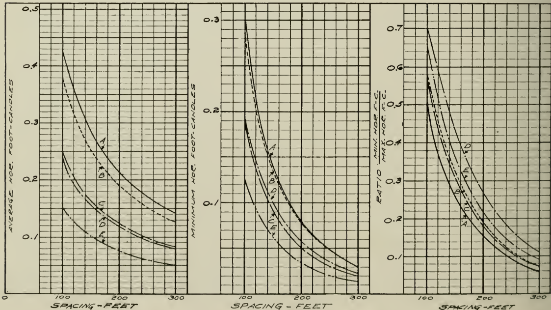
Fig. 11-c. Calculated Illumination Values on Street Surface along Center Line of Street Lamps on one side of street only, on 1-ft. bracket arm. Height, 25 ft. Width of street, 60 ft. A: 6.6-amp. long life electrode C: 5-amp. long life electrode B: 5-amp. high efficiency electrode D: 4-amp. high efficiency electrode E: 4-amp. long life electrode
