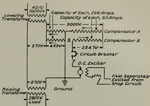
Fig. 4. A current-limiting reactor set-up employing two single-phase compensators with primaries excited by direct current
